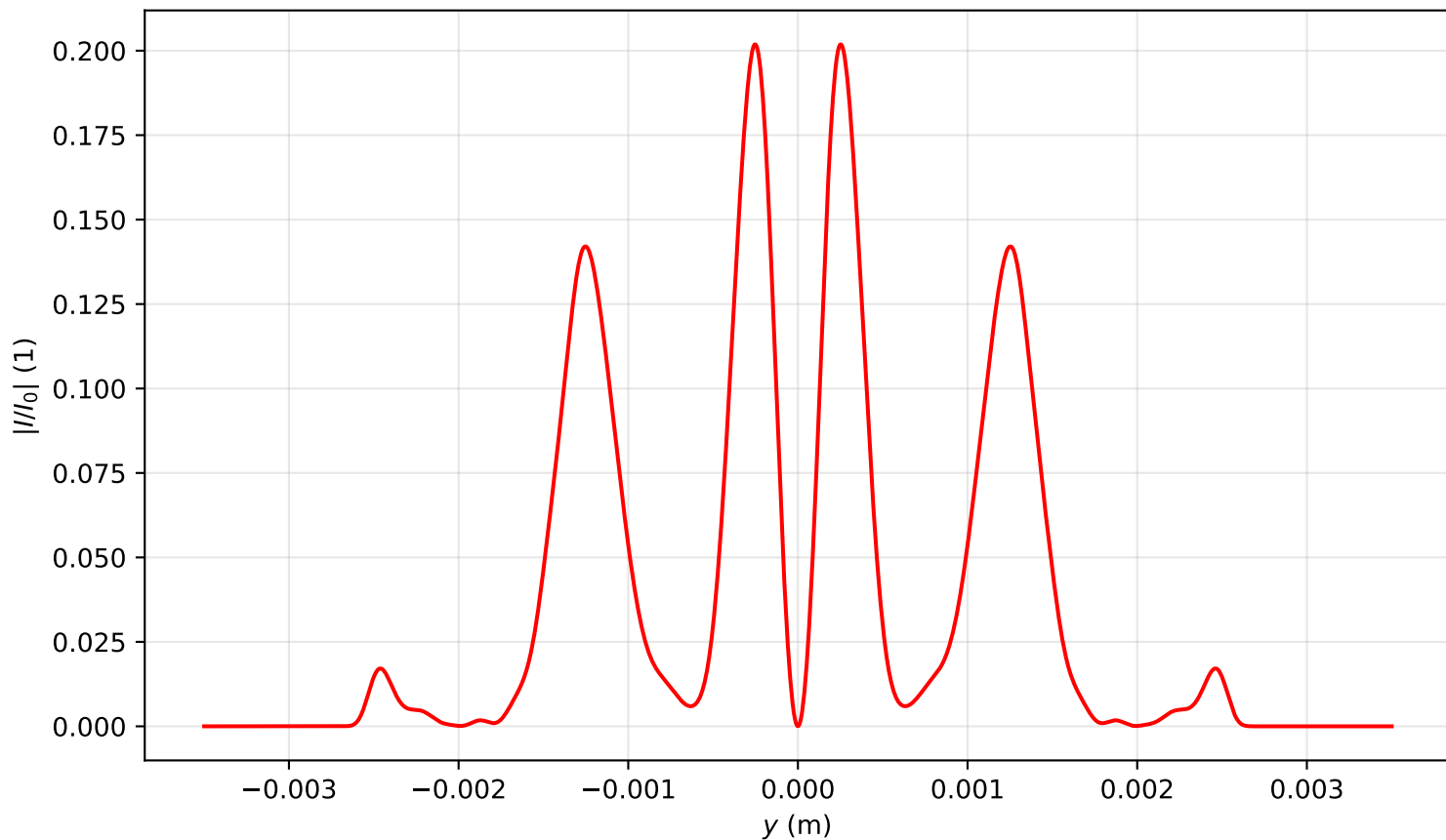
Intensity profile I(x=0, y, z=1.990)/I_0 , \text{Pin}=9.0\text{Pcr} , artificial time
